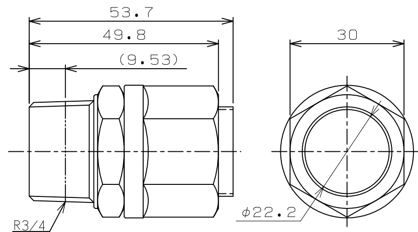
TITLE KADOMILESS KANTOUCH MODEL JH15-3/4-B-N-Ro
