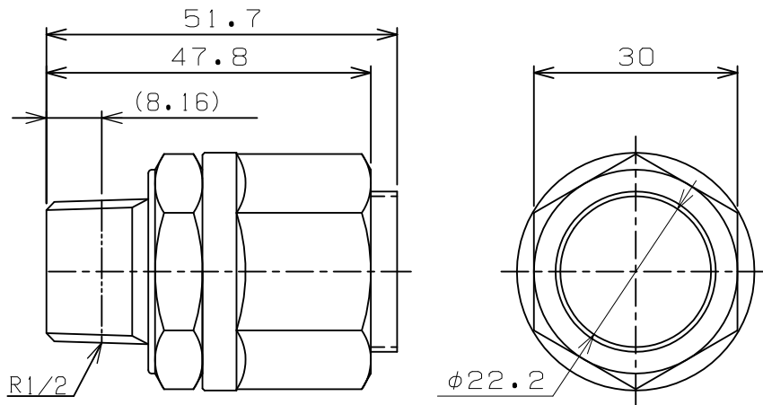
TITLE KADOMILESS KANTOUCH MODEL JH15-1/2-B-N-Ro
