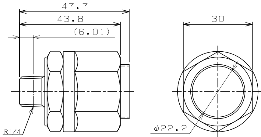
TITLE KADOMILESS KANTOUCH MODEL JH15-1/4-B-N-Ro
