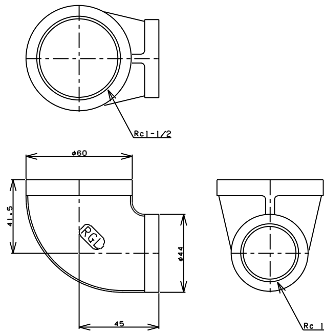
TITLE 径違い90°エルボ MODEL R-1A-1-1/2X1
