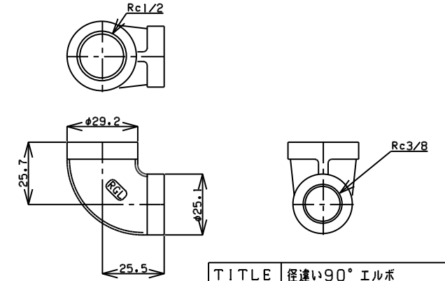
TITLE 径違い90°エルボ MODEL R-1A-1/2X3/8
