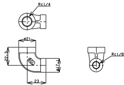
TITLE 径違い90°エルボ MODEL R-1A-1/4X1/8
