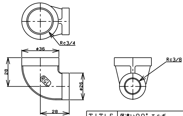
TITLE 径違い90°エルボ MODEL R-1A-3/4X3/8
