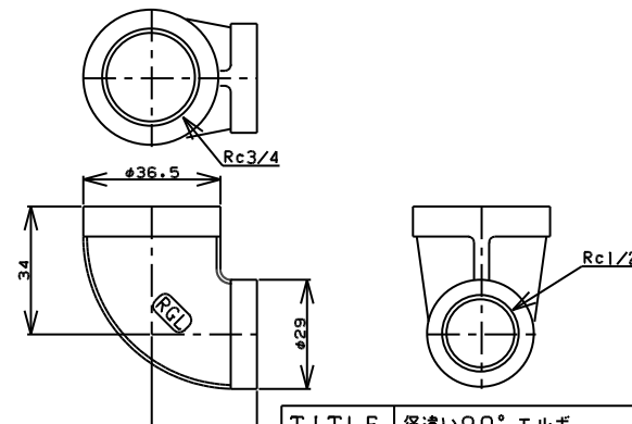
TITLE 径違い90°エルボ MODEL R-1A-3/4X1/2
