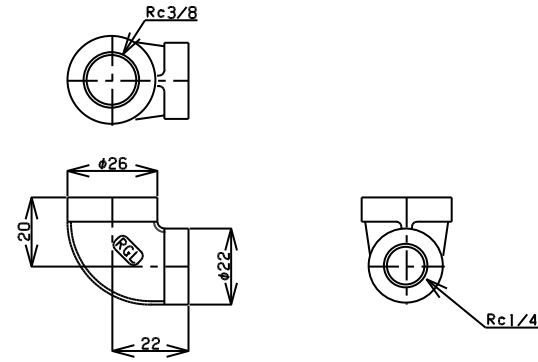
TITLE 径違い90°エルボ MODEL R-1A-3/8X1/4
