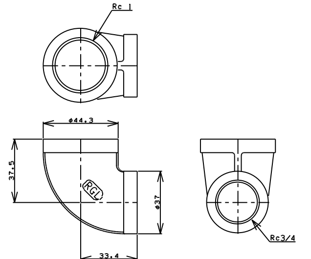
TITLE 径違い90°エルボ MODEL R-1A-1X3/4
