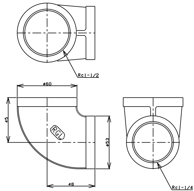
TITLE 径違い90°エルボ MODEL R-1A-1-1/2X1-1/4
