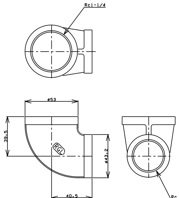
TITLE 径違い90°エルボ MODEL R-1A-1-1/4X1
