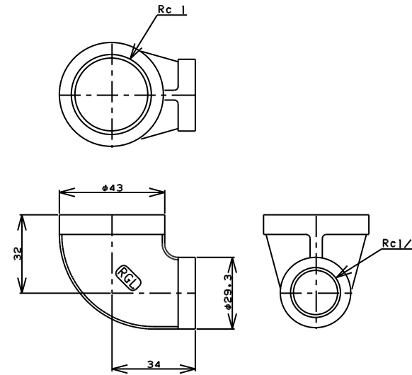
TITLE 径違い90°エルボ MODEL R-1A-1X1/2
