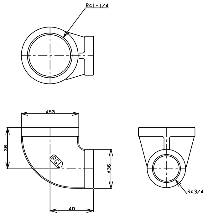
TITLE 径違い90°エルボ MODEL R-1A-1-1/4X3/4
