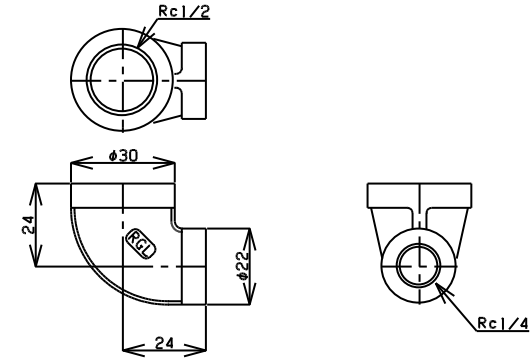
TITLE 径違い90°エルボ MODEL R-1A-1/2X1/4
